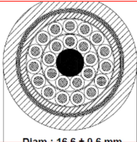
Diam : 16.6 ± 0.6 mm
